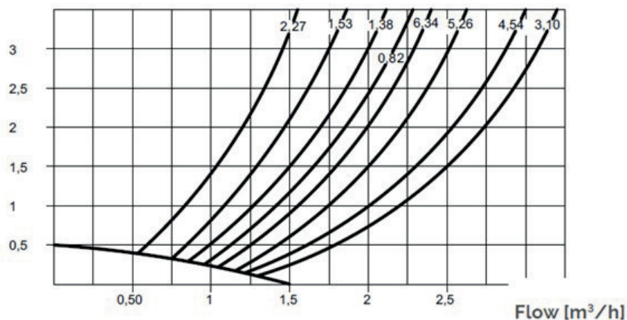
Pressure loss (mca)
